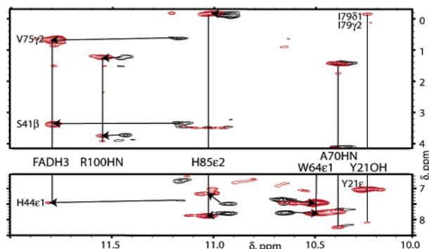
Figure 2. NOESY spectrum of unlabeled AppA5–125 in the dark (black) and light (red). Vertical bars highlight the light state resonances. Additional weak unassigned peaks appear in the light state.
