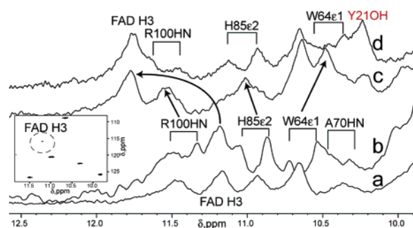
Figure 1. Region of 1 H NMR spectra of 15 N-labeled AppA5–125 with unlabeled FAD (a) in the dark using 15 N decoupling, (b) in the dark and 15 N-coupled, (c) illuminated (150 mW, 200 ms per 15 s) and 15 N-decoupled, and (d) illuminated and 15 N-coupled. All protein NH resonances are split by the 1 J NH coupling, while the unlabeled FAD H3 resonance is not. The Y21OH resonance at 10.22 ppm is not split and does not appear in HSQC spectra of the light-induced signaling state. Assignments of the resonances in the light-induced signaling state are indicated by arrows. The inset shows the HSQC spectrum of the same protein with 15 N-labeled FAD and a visible H3 resonance.
