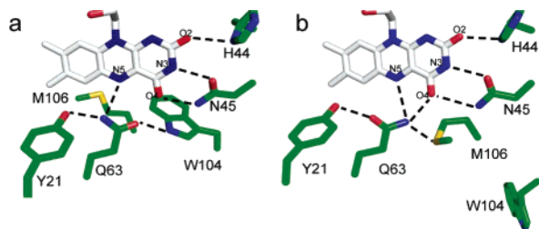
Figure 3. Dark state crystal structures of AppA (a) WT and (b) mutant C20S. The orientation of the Q63 side chain in (b) corresponds to the light-induced state of AppA proposed by Anderson et al. 11 except for the hydrogen bond to M106 (hydrogen bond distances shown as dotted lines).
